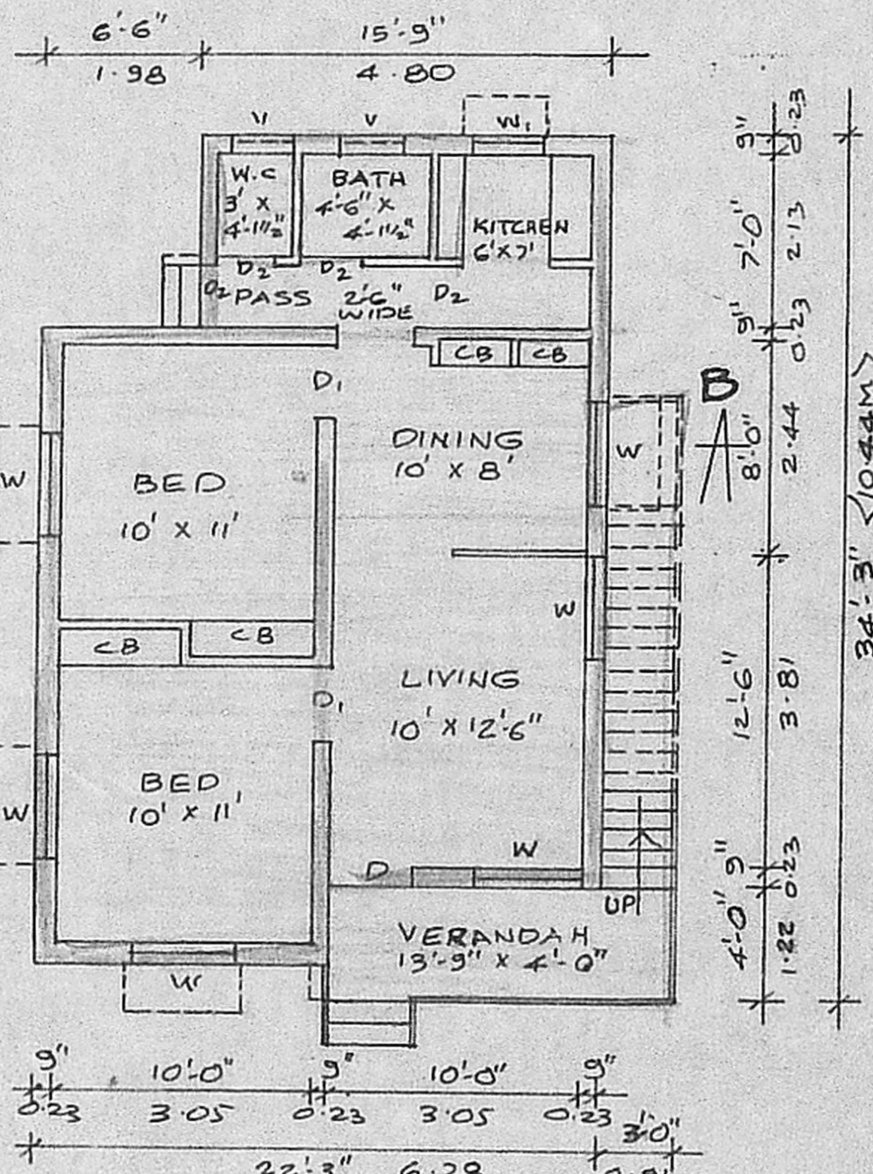
PLAN
