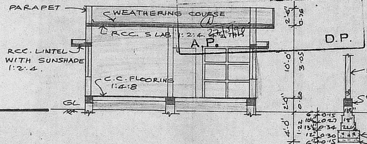
SECTION ON-AB
