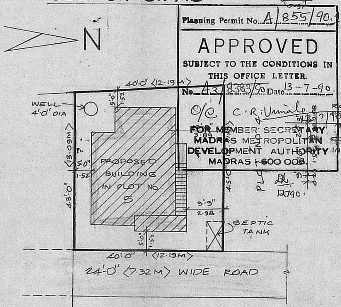
SITE PLAN
