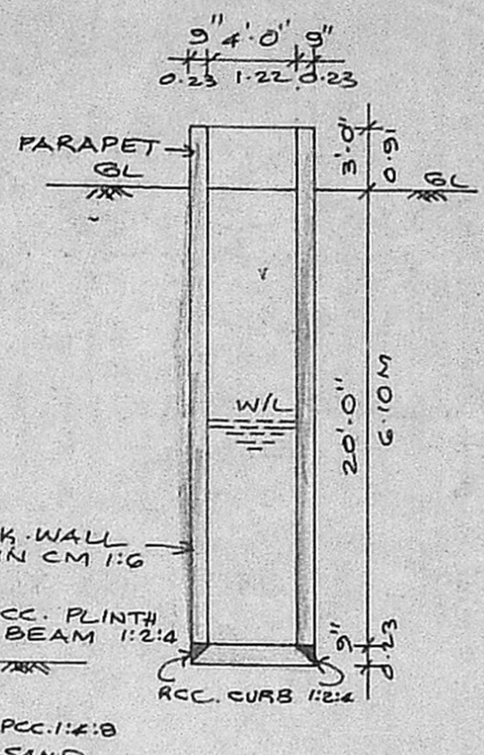
SECTION OF WELL 4'-0" DIA
